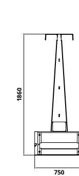
Cavalletto in lamiera zincata Zinc-plated sheet A-frame
